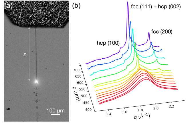
FIG. 1. (a) Stroboscopic image of the 3.5 \mu\text{m} -diameter krypton jet. The interaction with the focused x-ray beam resulted in plasma formation, visible as bright spot on the continuous filament, followed by vaporization of a segment of the jet. The trigger of the nanosecond laser-based background illumination was set to record an image of the jet after every fifth x-ray pulse. (b) Selection of azimuthally integrated and background-subtracted, powderlike diffraction profiles measured with the krypton jet. The labeled peaks represent reflections of the fcc and hcp crystal structures.
